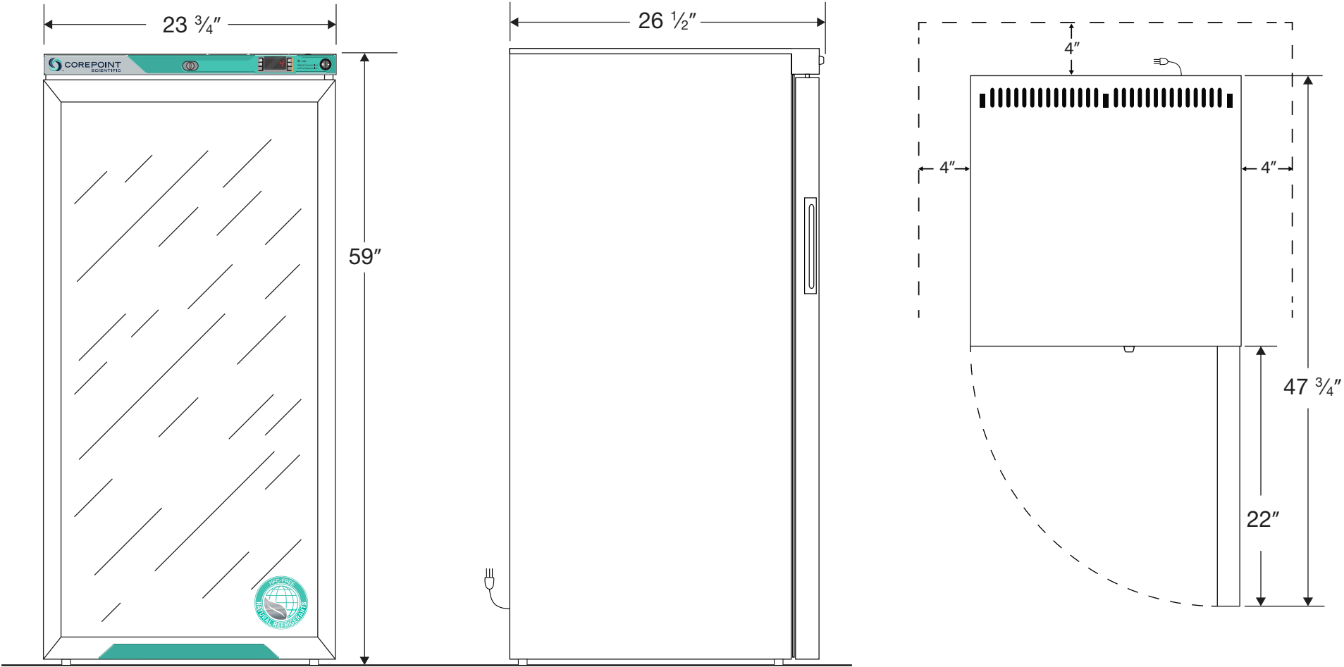
Front View
