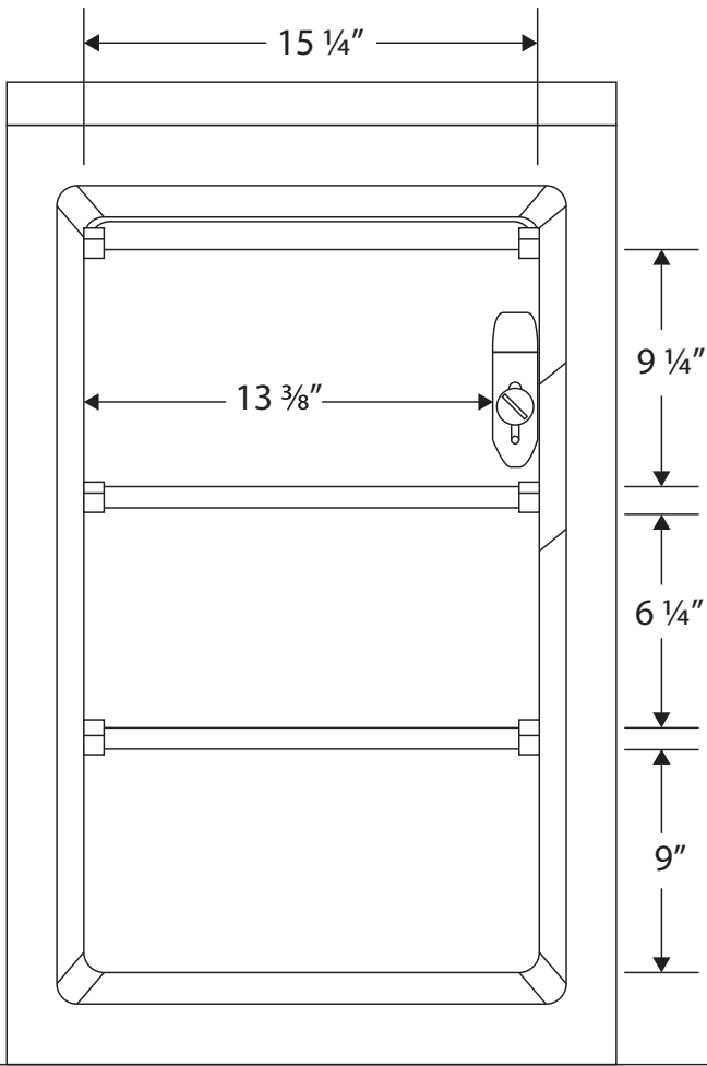
Front View
