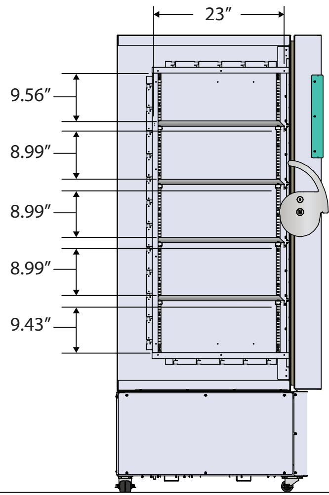
Side View
