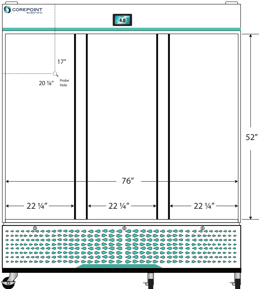
Front View
