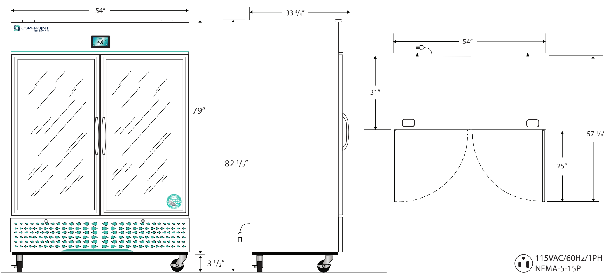
Front View
