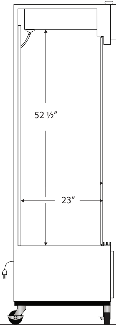
Side View
