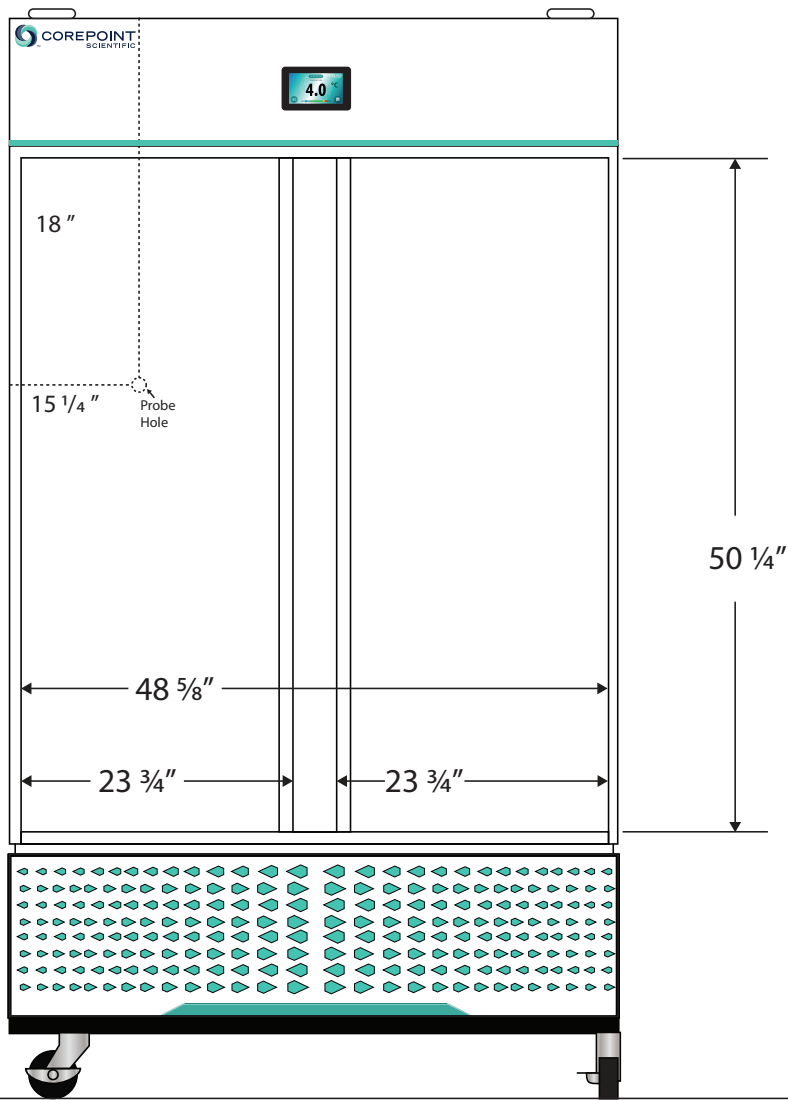
Front View
