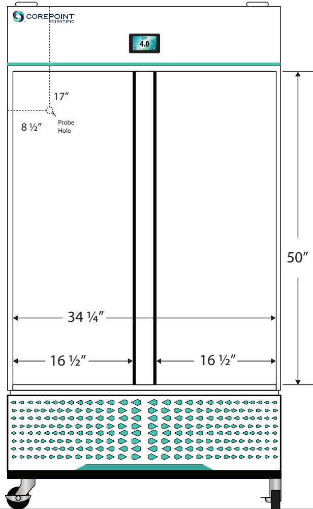
Front View
