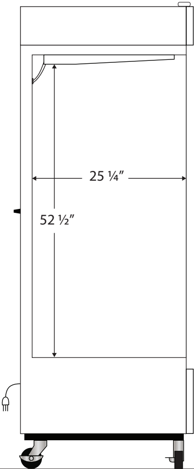
Side View
