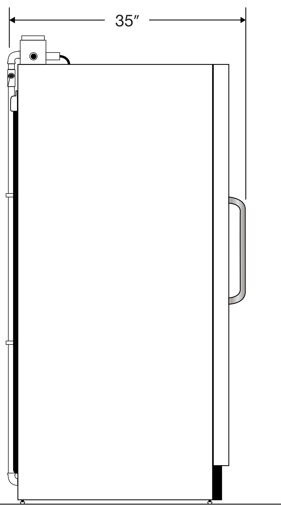
Side View
