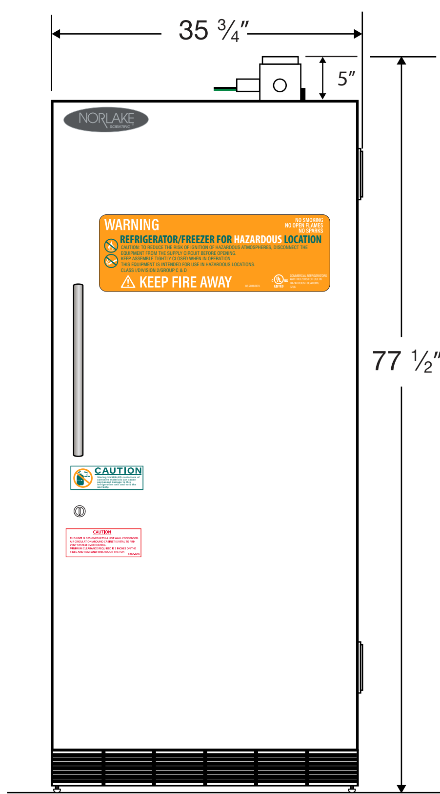
Front View
