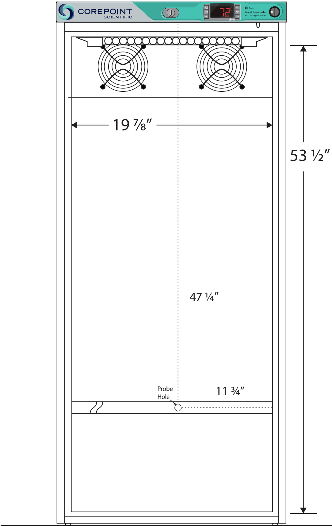
Front View
