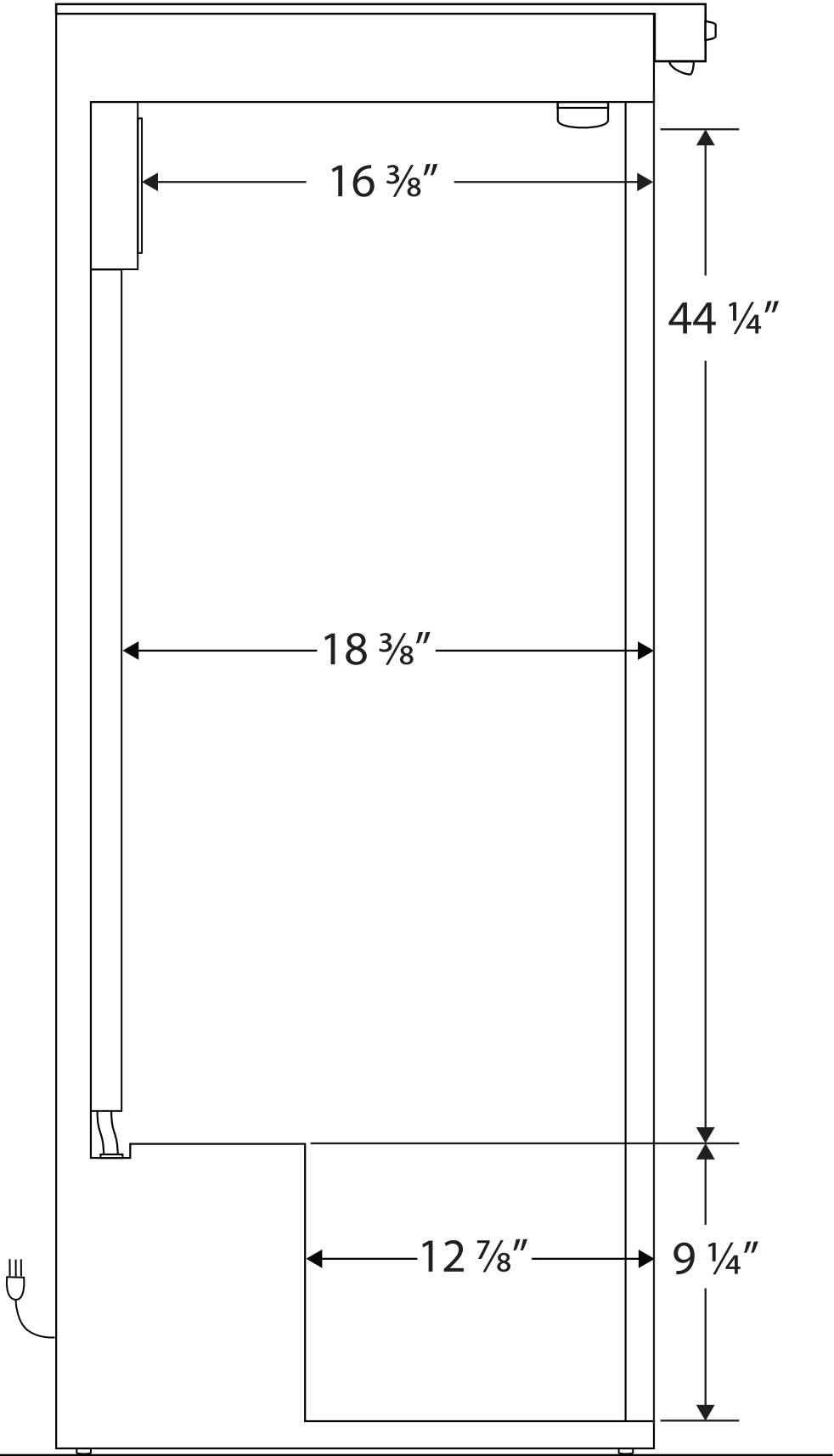
Side View
